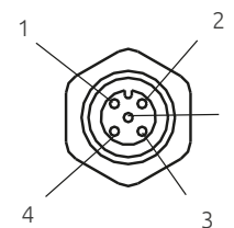
MUTING SENSOR M12-pole
